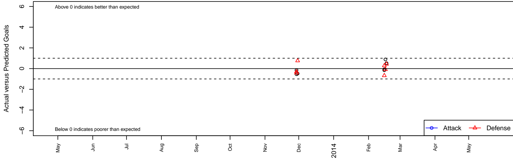
Albion SC Premier G99 Dots are actual minus expected GF (blue circles) and GA (red triangles). Blue line is smoothed change in attack strength. Red is smoothed change in defense strength.
